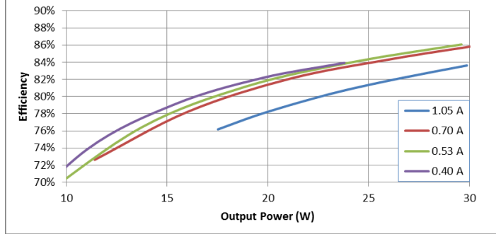
Efficiency Vs. Output Power, 277V In
