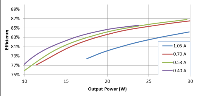
Efficiency Vs. Output Power, 120V In
