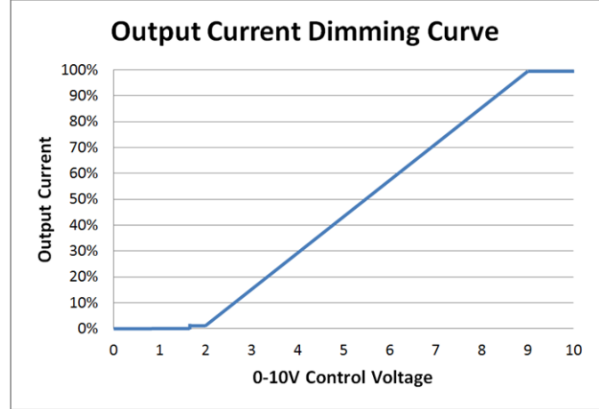
Linear Dimming w/ Dim-to-Off
